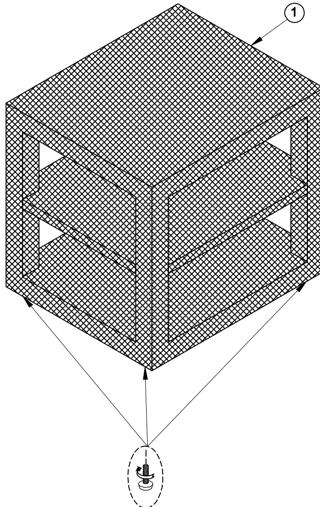
Adjustable leveler
